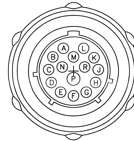
PIN VIEW/ FACE VIEW
